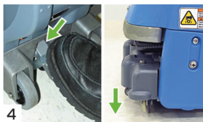
4 Lower scrubhead.
